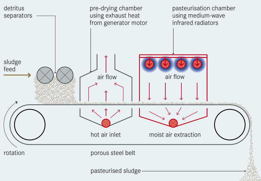
Figure 6: Schematic of the LaDePa sludge pelletizer
